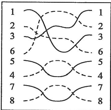
(c) 交叉线对
